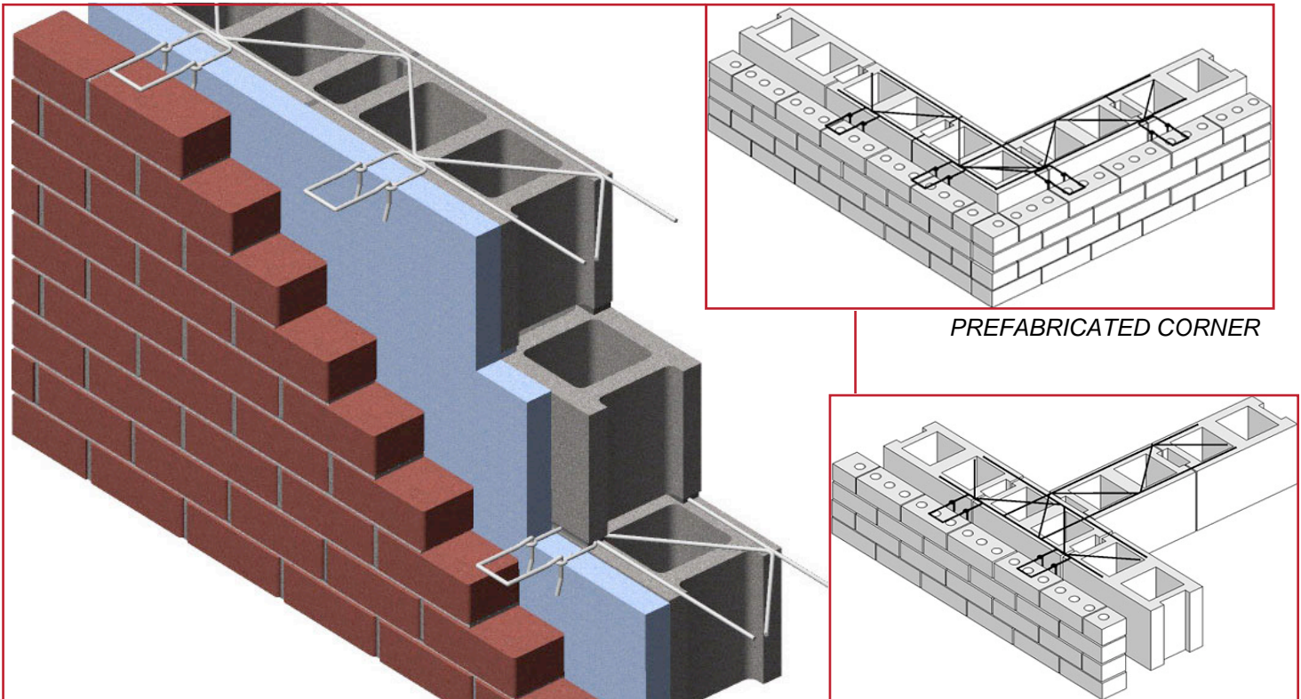
PREFABRICATED TEE
